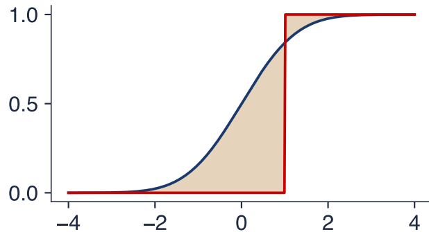
CRPS = 0.602
