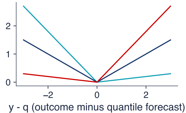
Pinball loss
