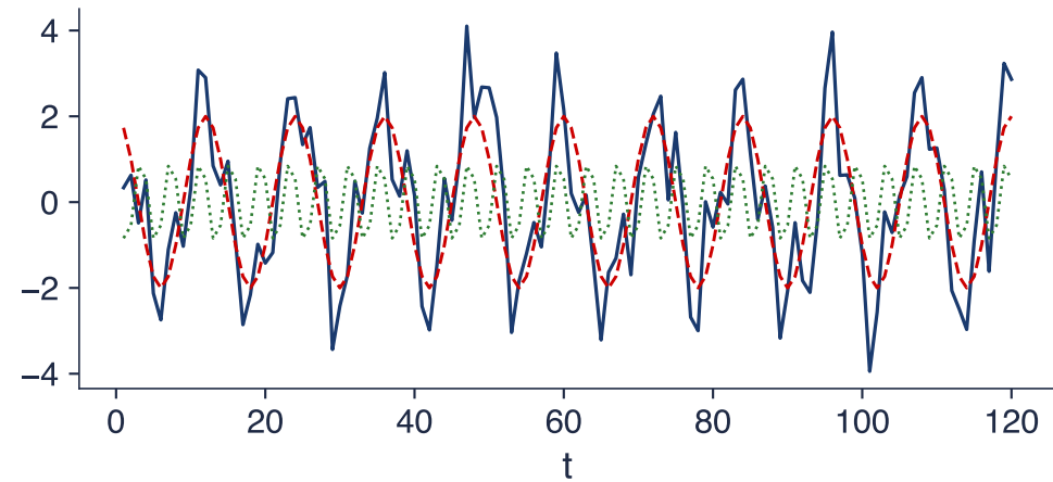
Two cycles plus noise
