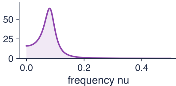
AR(2), \phi = (1.5, -0.75)
