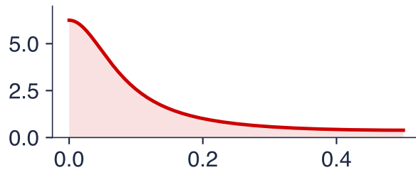
AR(1), \phi = 0.6
