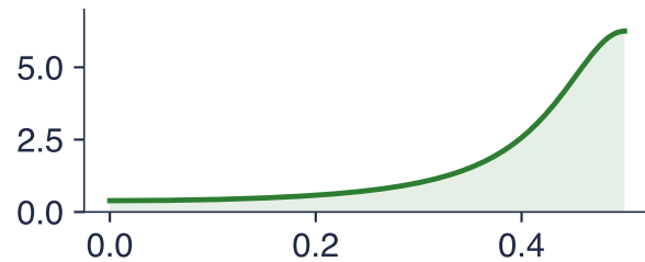
AR(1), \phi = -0.6
