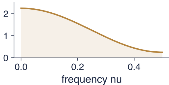
MA(1), \theta = 0.5
