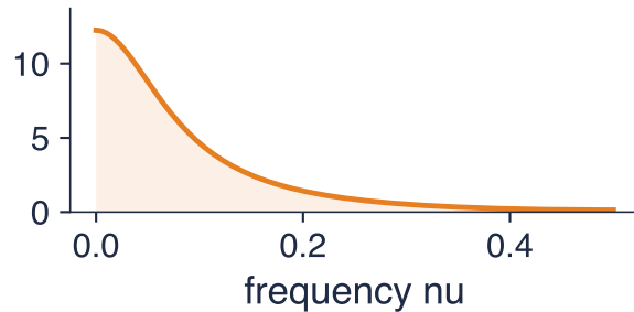
ARMA(1,1), \phi = 0.6 , \theta = 0.4
