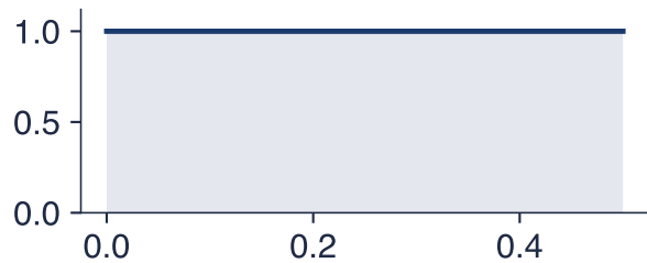
white noise
