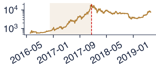
Bitcoin, 2017
