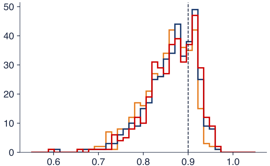
AR(1), \phi = 0.9 , T = 100 : 400 samples
