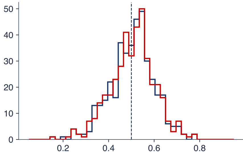
MA(1), \theta = 0.5 , T = 100 : conditional LS and ML
