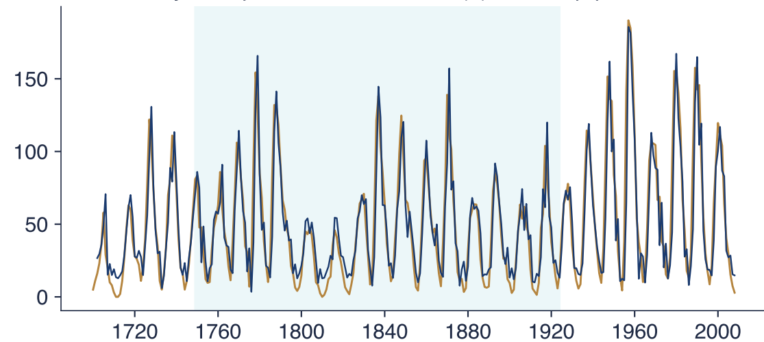
Yearly sunspot numbers and AR(2) one-step predictions
