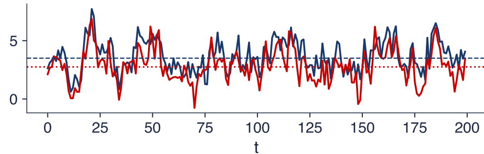
Simulated VAR(1), T = 200
