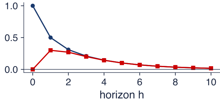
Impulse responses \Phi_h = A^h
