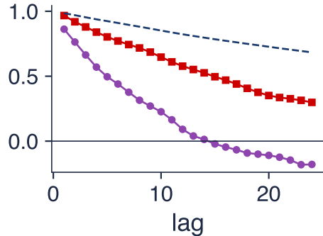
Sample ACF
