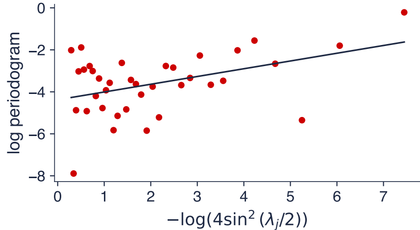
RO inflation (monthly, SA): d = 0.37 (SE 0.11), m = 37
