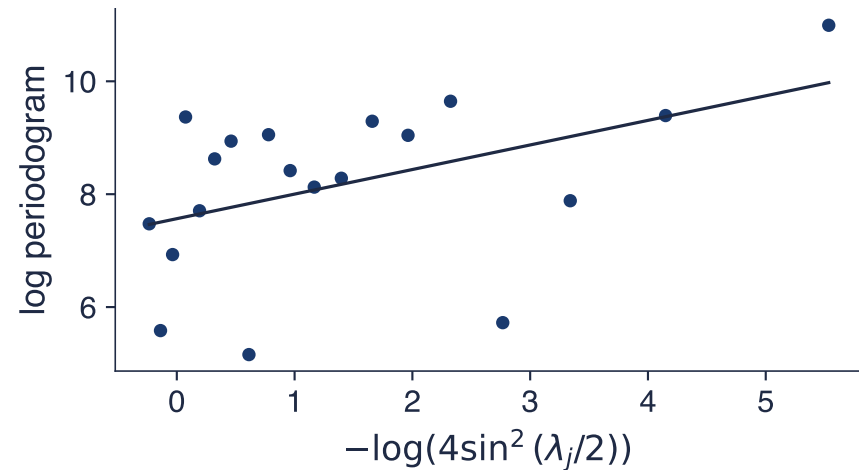
Nile flow: d = 0.44 (SE 0.15), m = 19
