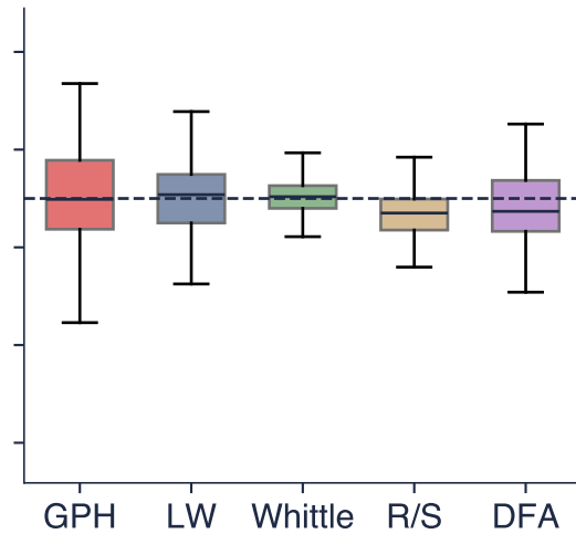
ARFIMA(0,0.3,0), d = 0.3
