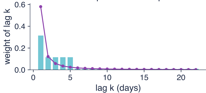
HAR: three steps that mimic a power law
