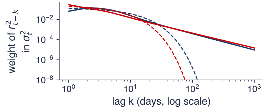
ARCH( \infty ) weights
