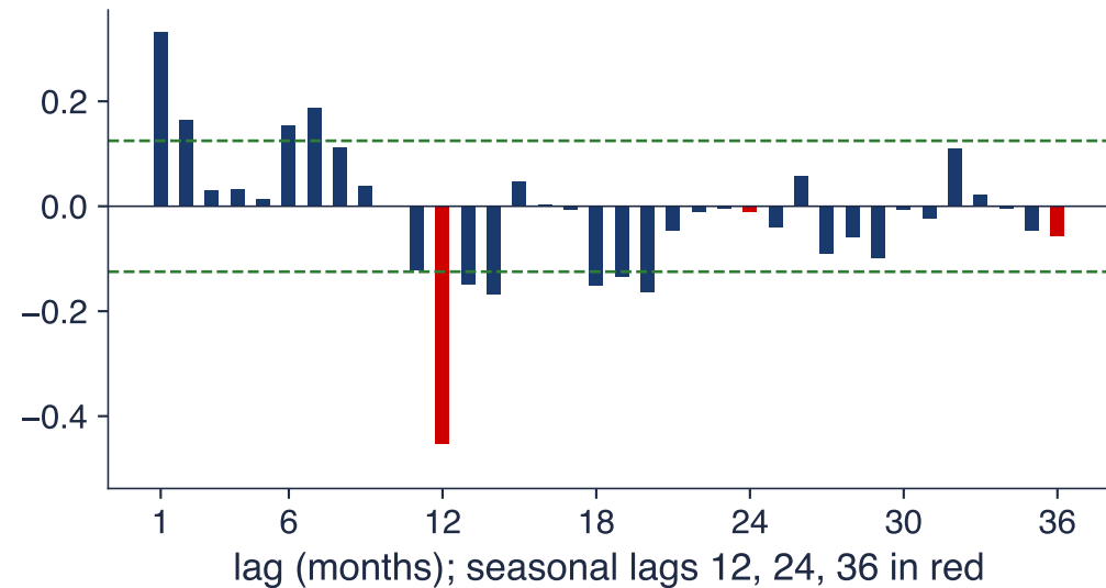
ACF of z = \Delta\Delta 12 \ln P
