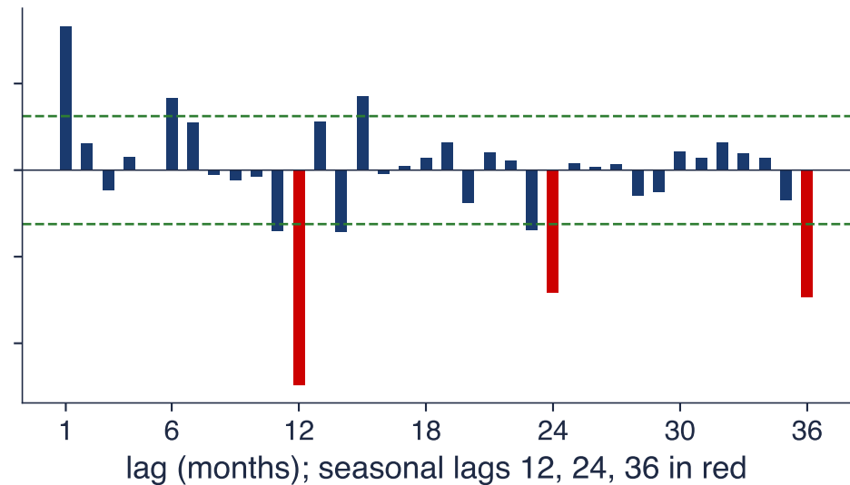
PACF of z = \Delta\Delta 12 \ln P
