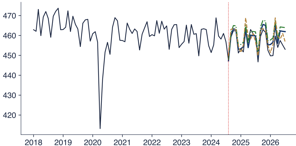
industrial production of Romania: test sample forecasts
