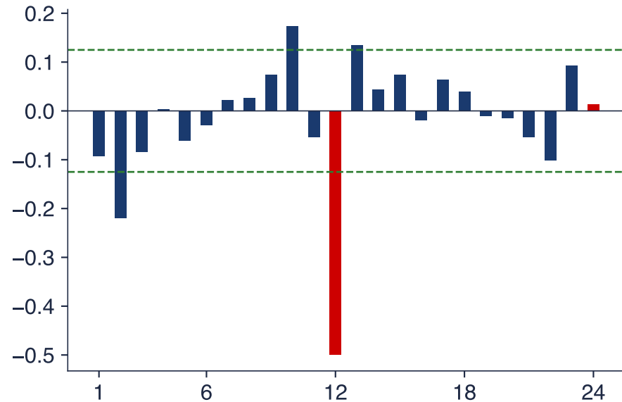
ACF of \Delta\Delta_{12} \ln IP
