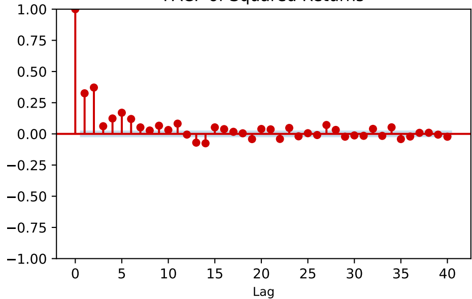
PACF of Squared Returns
