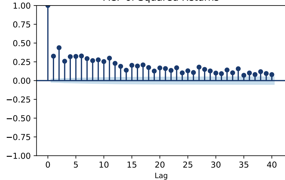
ACF of Squared Returns
