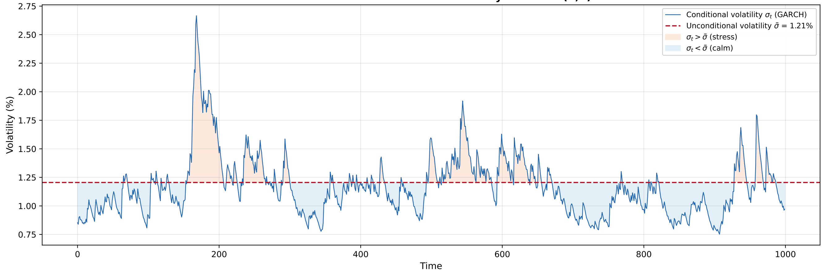
Conditional vs Unconditional Volatility — GARCH(1,1)
