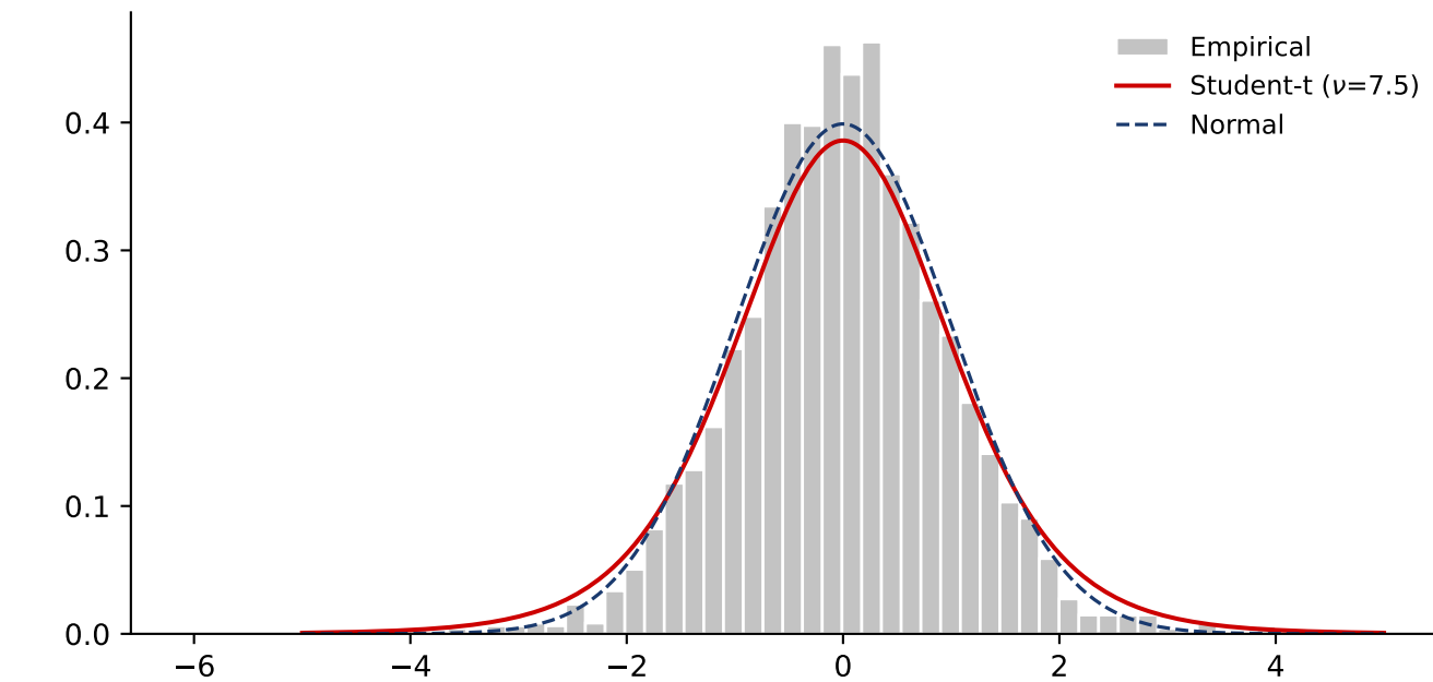
(c) Distribution of \hat{z}_t
