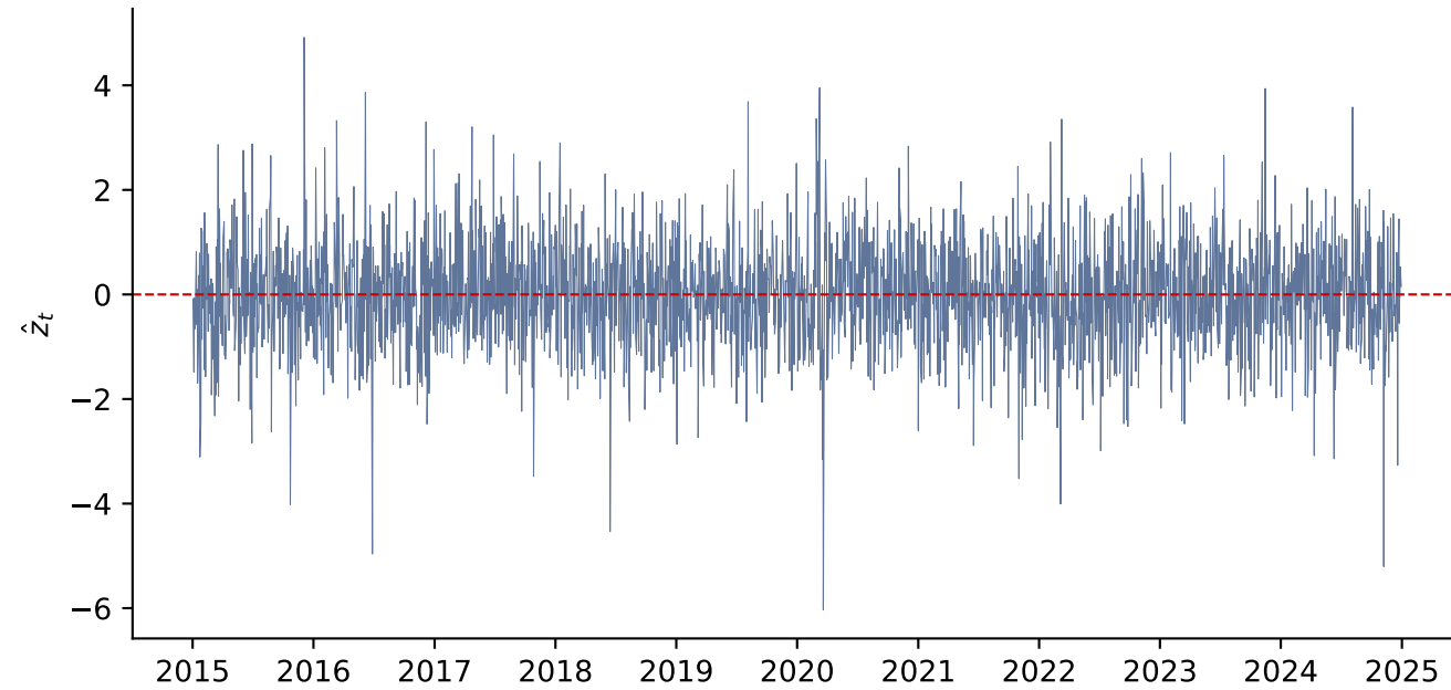
(a) Standardized Residuals \hat{z}_t
