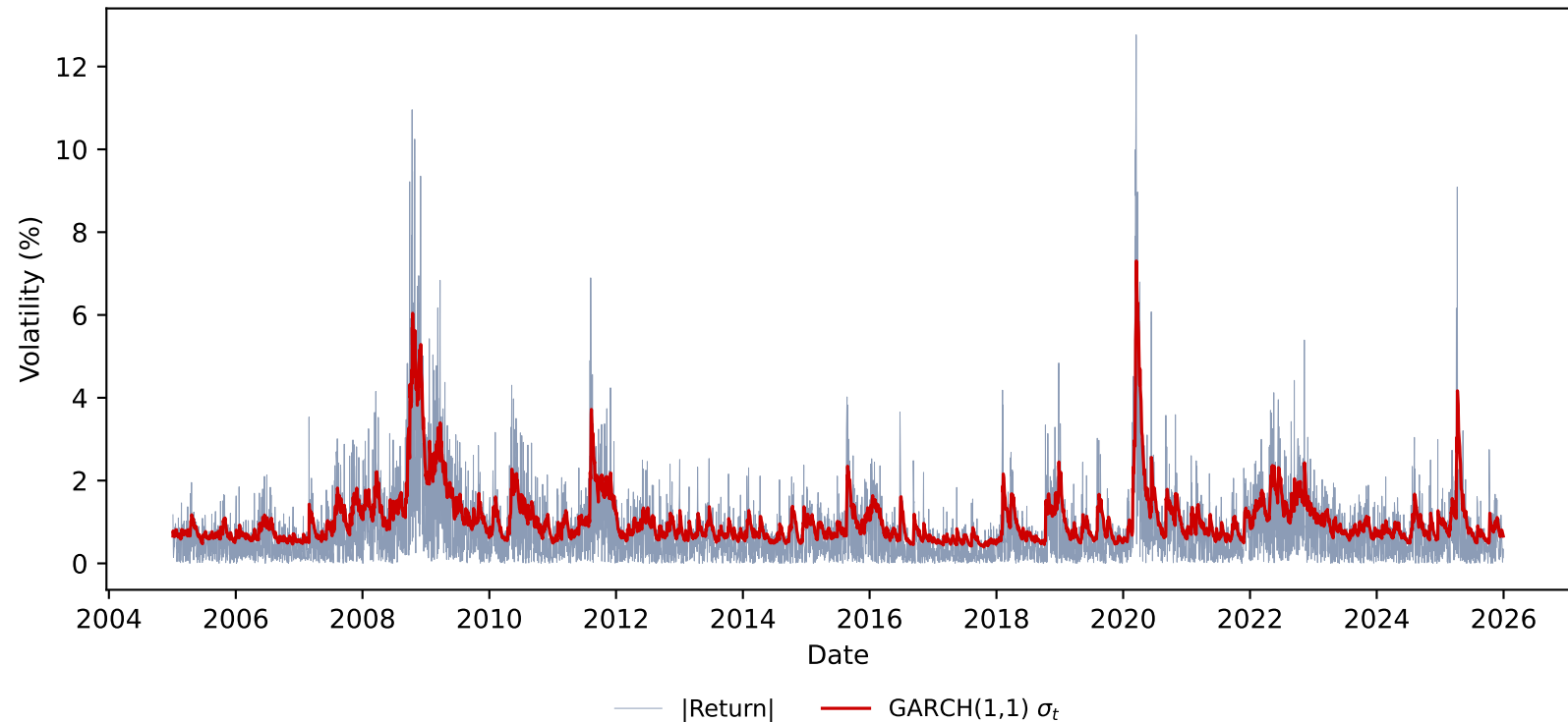
GARCH(1,1) Conditional Volatility vs Absolute Returns
