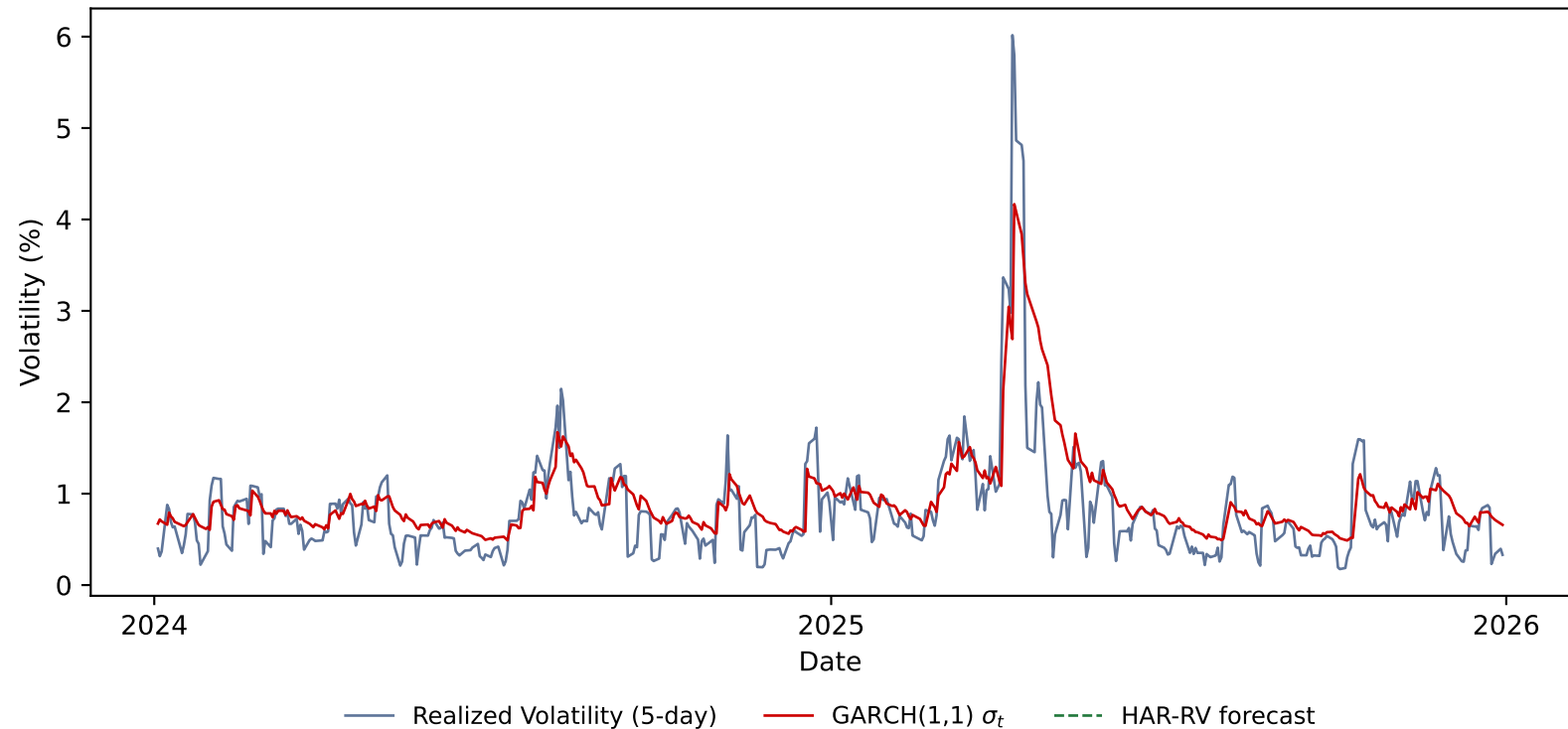
HAR-RV vs GARCH Volatility Comparison
