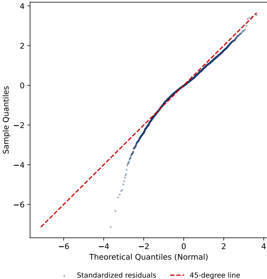
QQ-Plot of GARCH(1,1) Standardized Residuals
