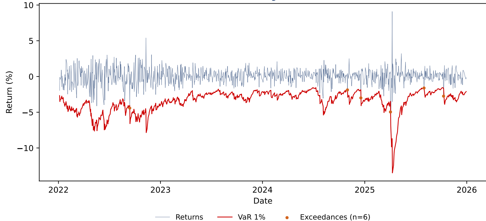
VaR(1%) Backtesting — GARCH(1,1)
