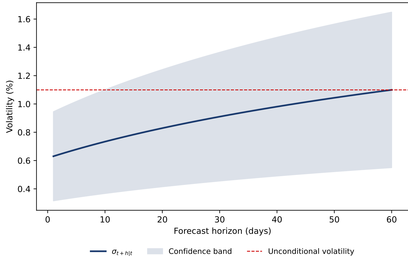
GARCH(1,1) Multi-Step Volatility Forecast
