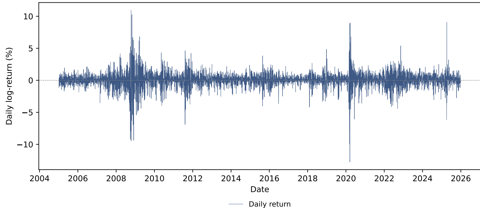
S&P 500 Daily Returns — Volatility Clustering
