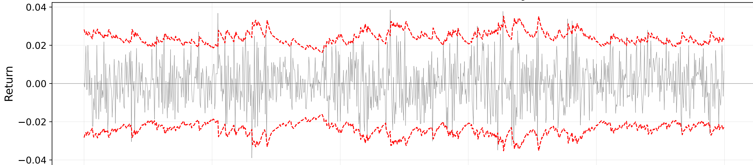
CGARCH: Simulated returns with volatility bands
