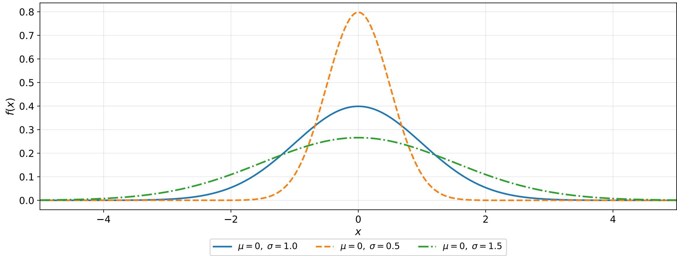
Normal Distribution — PDF
