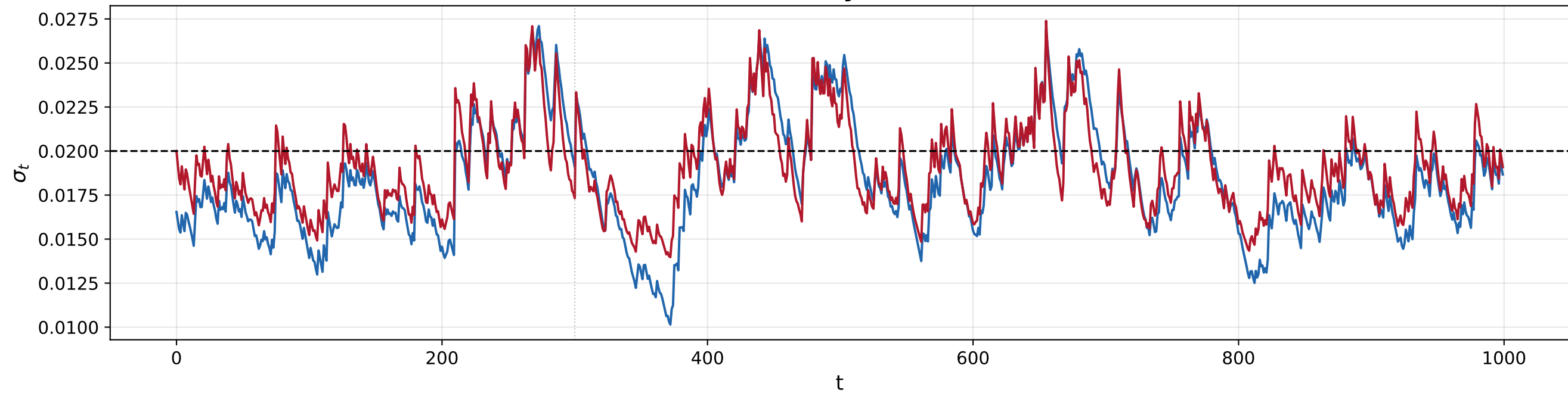
Conditional volatility: EWMA vs GARCH
