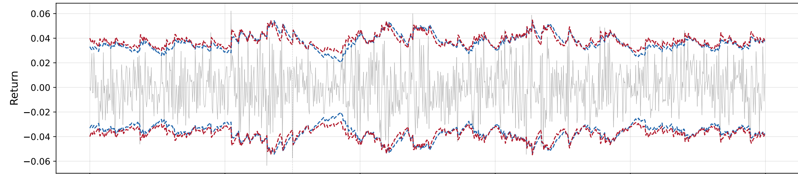
Simulated returns with EWMA (blue) vs GARCH (red) bands
