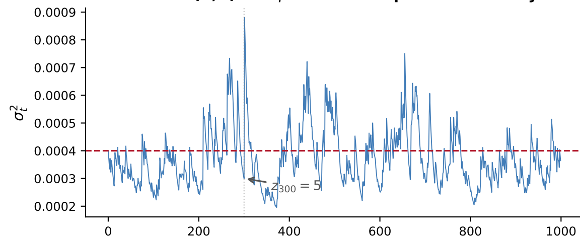
GARCH(1,1): \alpha + \beta = 0.95 — exponential decay
