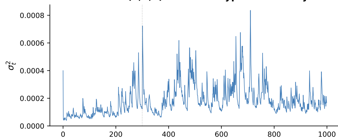
FIGARCH(1,d,1): d = 0.4 — hyperbolic decay
