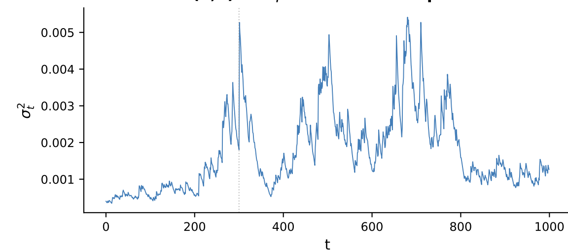
IGARCH(1,1): \alpha + \beta = 1.0 — infinite persistence
