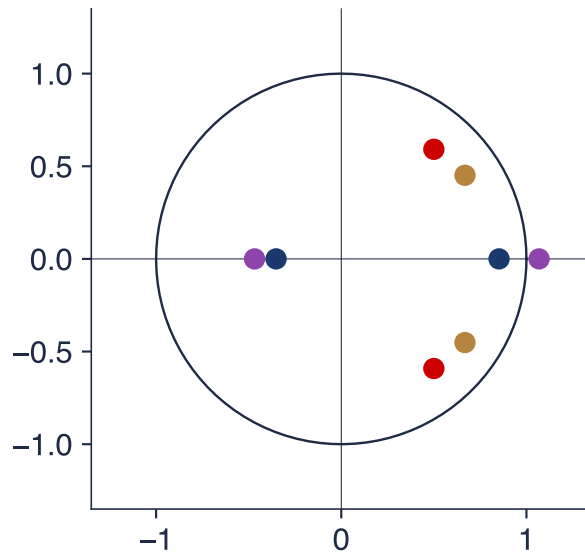
Inverse roots and the unit circle
