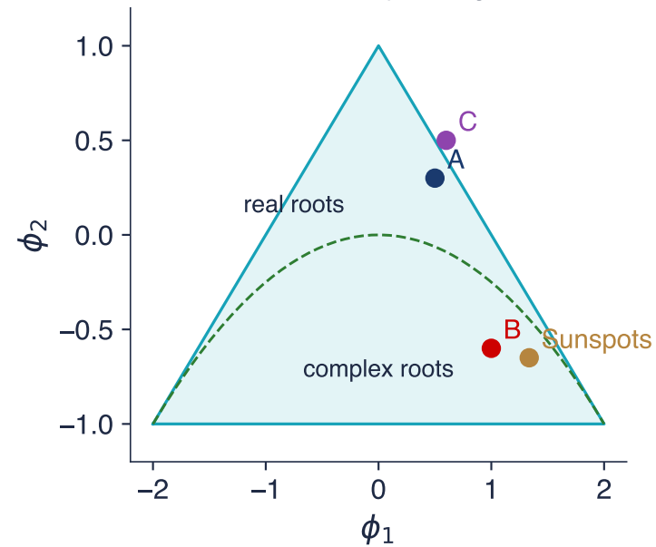
Stationarity triangle
