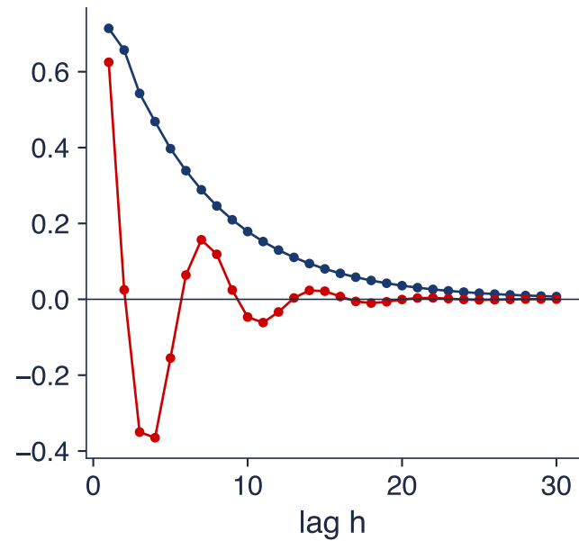
Theoretical ACF of A and B
