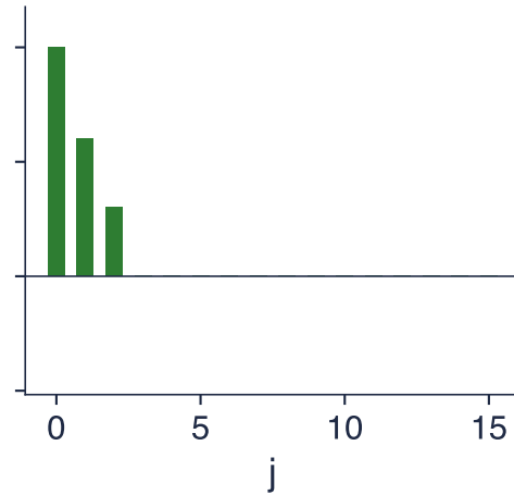
MA(2), \theta = (0.6, 0.3)
