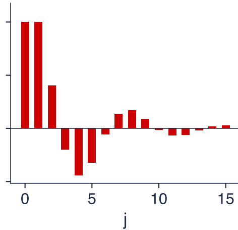
AR(2), \phi = (1.0, -0.6)
