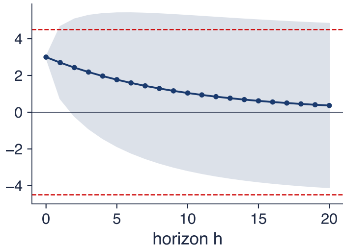
AR(1), \phi = 0.9
