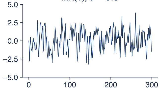
MA(1), \theta = 0.8
