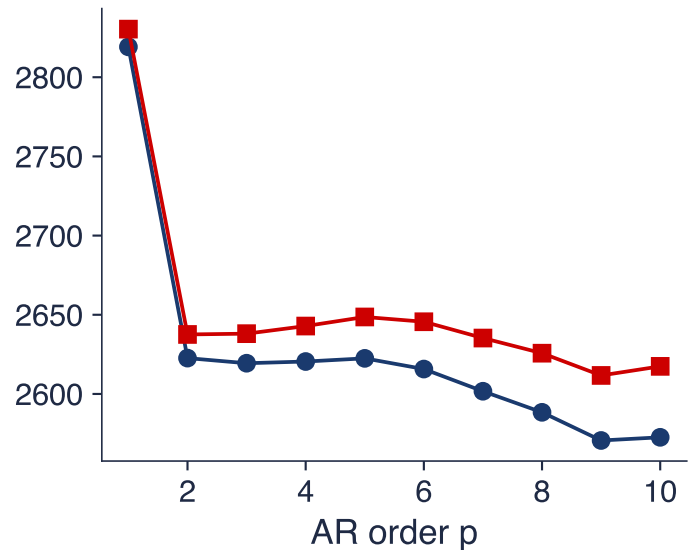
Information criteria, full sample
