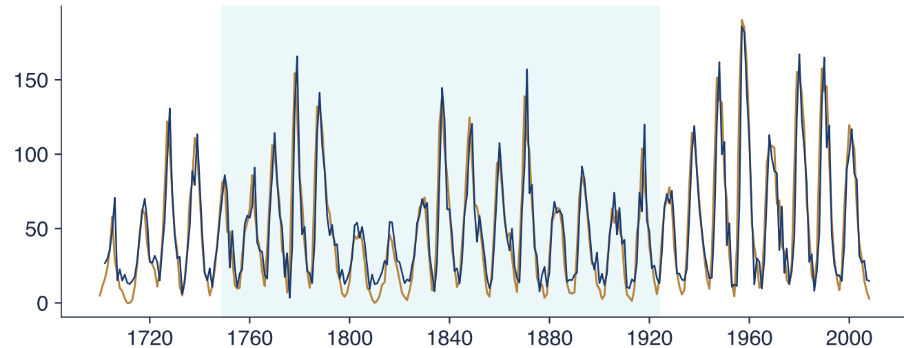
Yearly sunspot numbers and AR(2) one-step predictions
