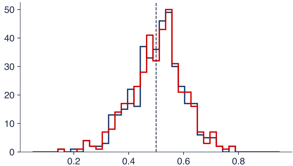
MA(1), \theta = 0.5 , T = 100 : conditional LS and ML
