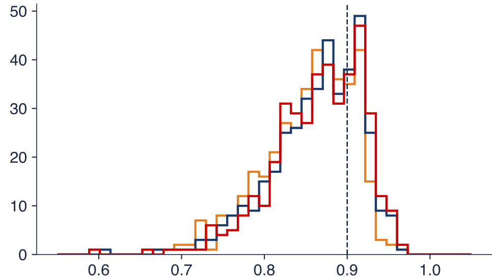
AR(1), \phi = 0.9 , T = 100 : 400 samples
