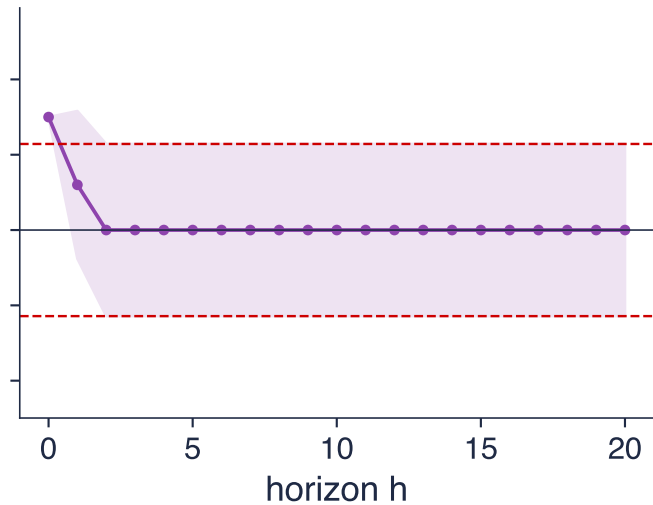
MA(1), \theta = 0.6 , \varepsilon_T = 2
