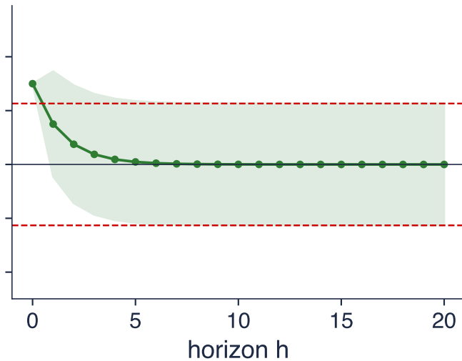
AR(1), \phi = 0.5
