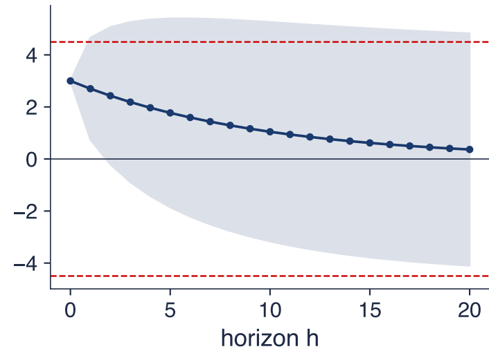
AR(1), \phi = 0.9
