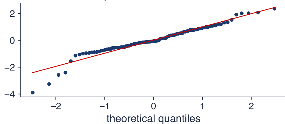
Normal QQ plot of the standardised residuals
