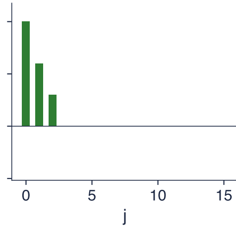
MA(2), \theta = (0.6, 0.3)
