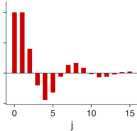
AR(2), \phi = (1.0, -0.6)
