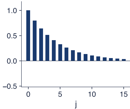
AR(1), \phi = 0.8
