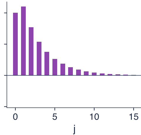
ARMA(1,1), \phi = 0.7, \theta = 0.4
