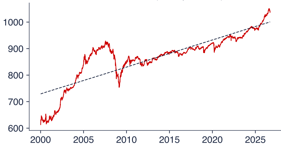
BET: 100 ln P (ADF \rho = 0.65 )
