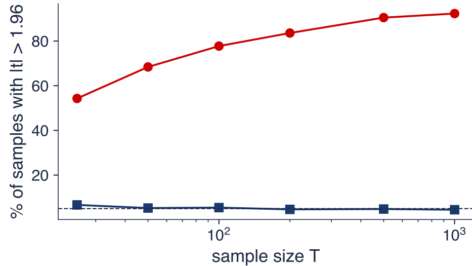
Rejection rate of a true null
