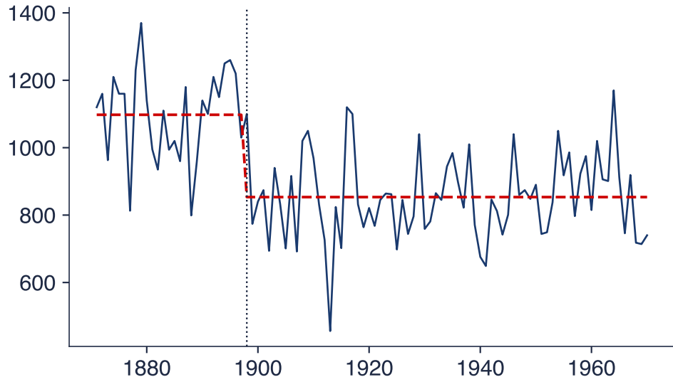
Nile flow: break in 1898, ZA = -6.86
