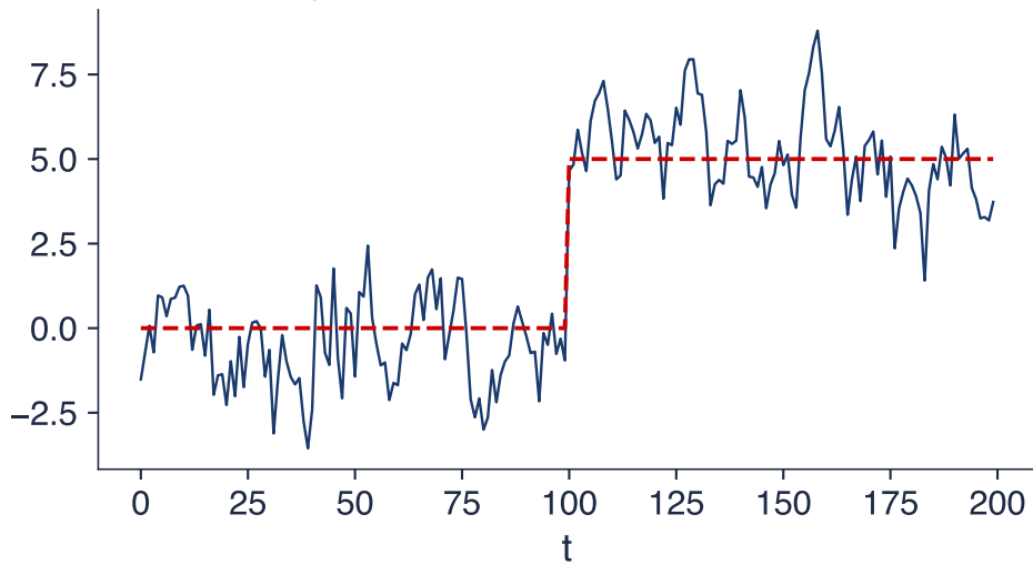
Stationary around a broken mean: ADF p = 0.17
