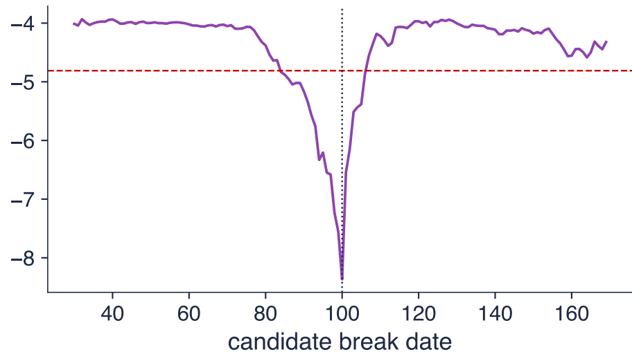
Zivot-Andrews: search over break dates
