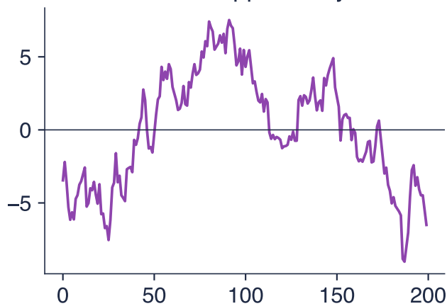
Residuals: apparent cycles
