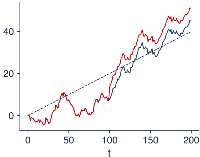
Difference-stationary: y_t = 0.2 + y_{t-1} + \varepsilon_t
