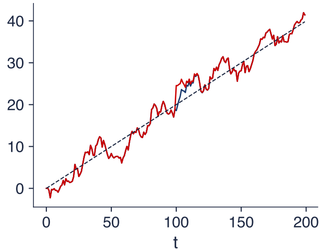
Trend-stationary: y_t = 0.2 t + u_t
