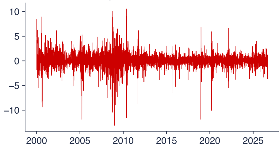
Daily log returns, % (ADF = -16.5)
