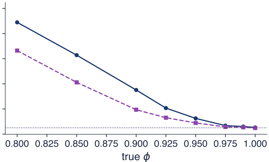
T = 100: an unnecessary trend costs power
