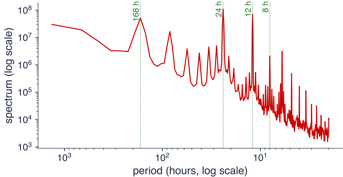
Spectrum of the hourly load
