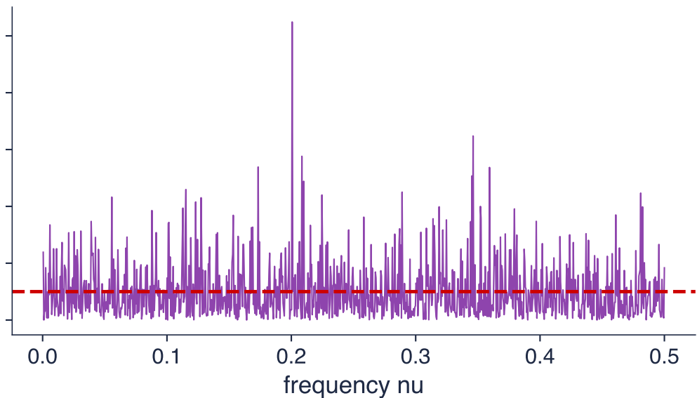
White noise, T = 2048
