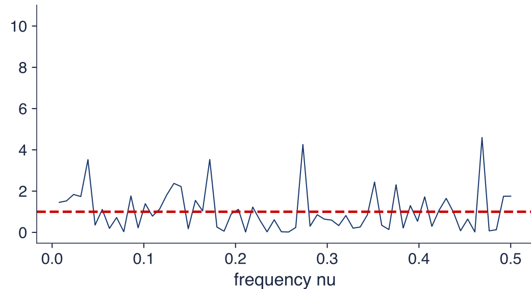
White noise, T = 128
