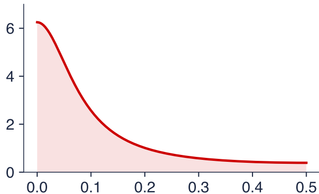
AR(1), \phi = 0.6
