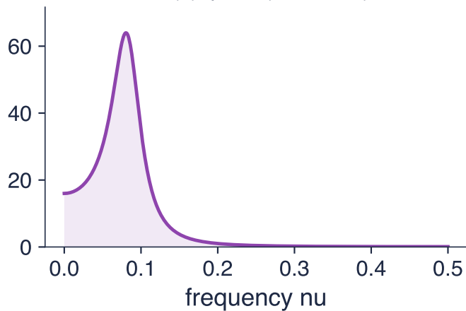
AR(2), \phi = (1.5, -0.75)
