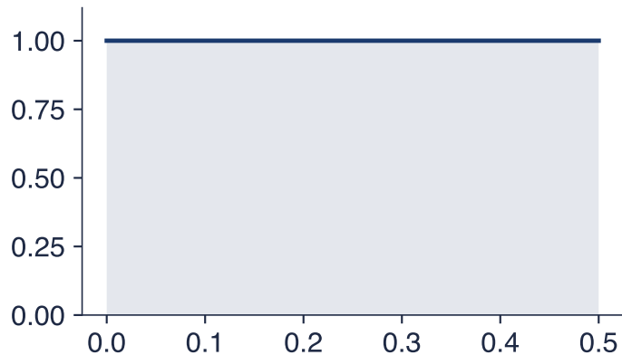
white noise
