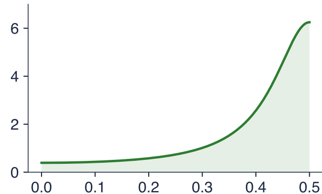
AR(1), \phi = -0.6
