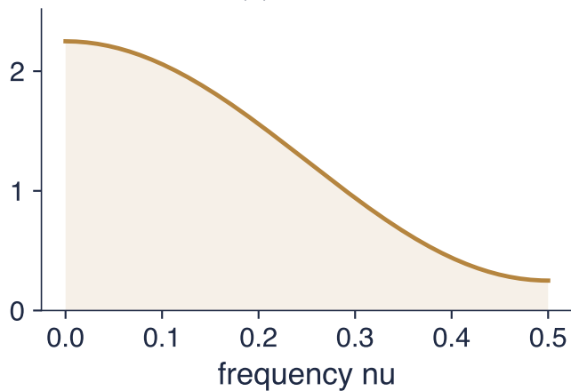
MA(1), \theta = 0.5
