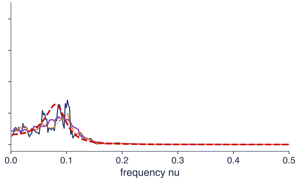
Smoothed estimates
