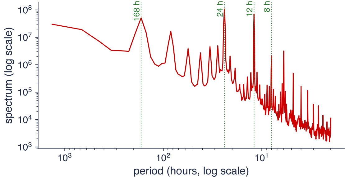
Spectrum of the hourly load
