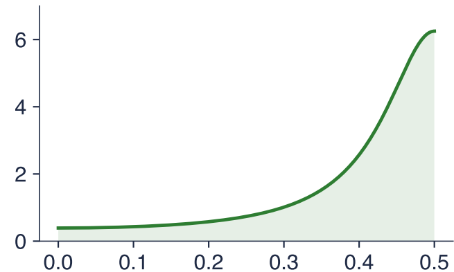
AR(1), \phi = -0.6
