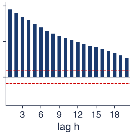
Random walk
